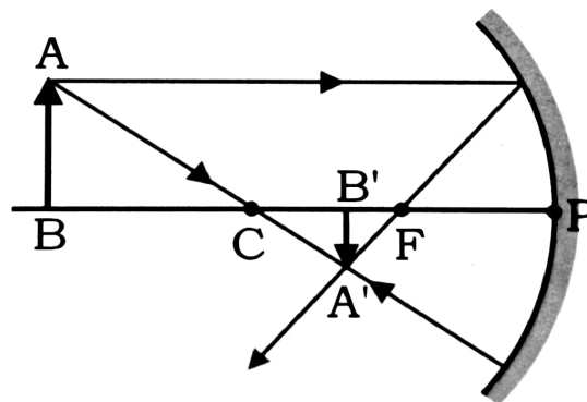
Object beyond Center of Curvature
