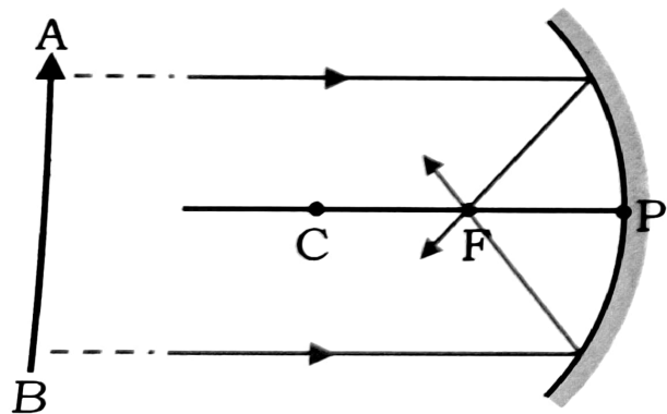
Object at infinity
